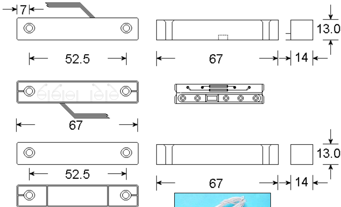
Magnet
